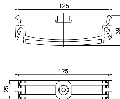
Clip Nylon
