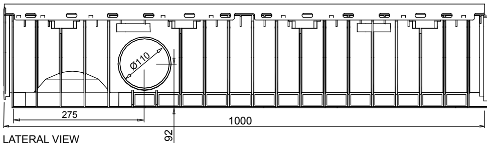
LATERAL VIEW
