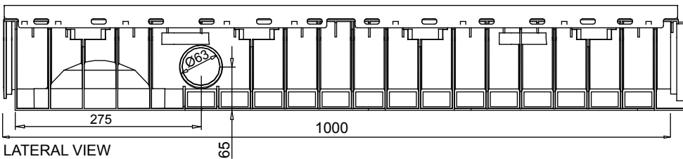
LATERAL VIEW
